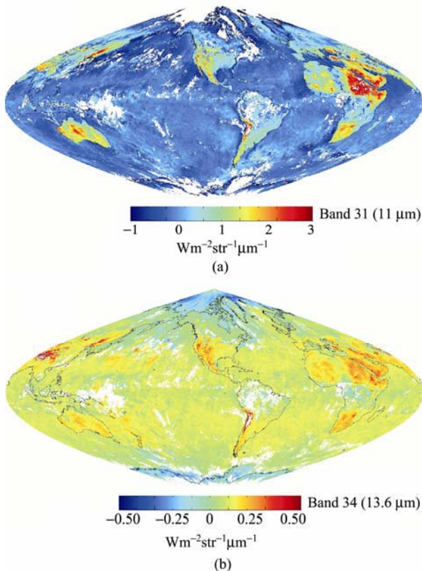
Figure 5.6 Two examples of mean daytime Terra 8-day biases are shown: (a) 11 \mu\text{m} (Band 31) and (b) 13.6 \mu\text{m} (Band 34). Notice that in the Band 31 example, large differences occur over land surfaces where diurnal heating is not adequately captured by input surface temperatures. The Band 34 example indicates that perhaps upper tropospheric temperatures or tropopause locations were not accurate in this time period (April 1 – 8, 2003). Figures depict observed minus calculated radiances
