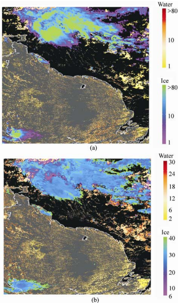
Figure 5.3 (a) Retrieved cloud optical thickness and (b) effective particle size for both ice- and water-phase clouds at 1-km spatial resolution for the scene in Fig. 5.1
