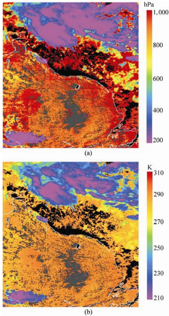
Figure 5.2 (a) Retrieved cloud-top pressure in hPa and (b) cloud-top temperature in Kelvin obtained at 5-km spatial resolution for the scene in Fig. 5.1
