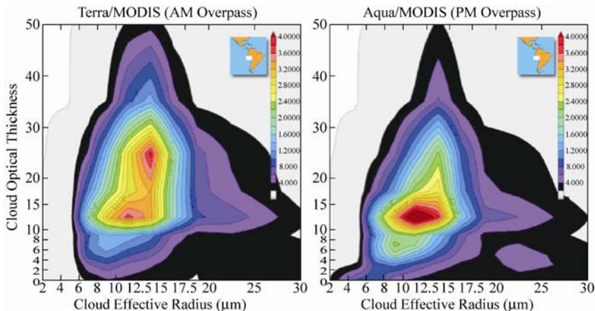
Figure 5.5 Joint histogram of liquid water cloud optical thickness and effective particle size from products derived in August 2003, between 10^{\circ} - 20^{\circ} S, 70^{\circ} - 85^{\circ} W (coastal Peru/Chile)
