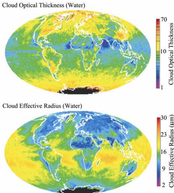
Figure 5.4 MODIS Terra Level-3 April 2003 monthly aggregations for liquid water cloud retrievals of optical thickness (top) and effective particle radius (bottom)
